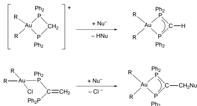
Scheme 1 \text{R} = \text{C}_6\text{F}_5
